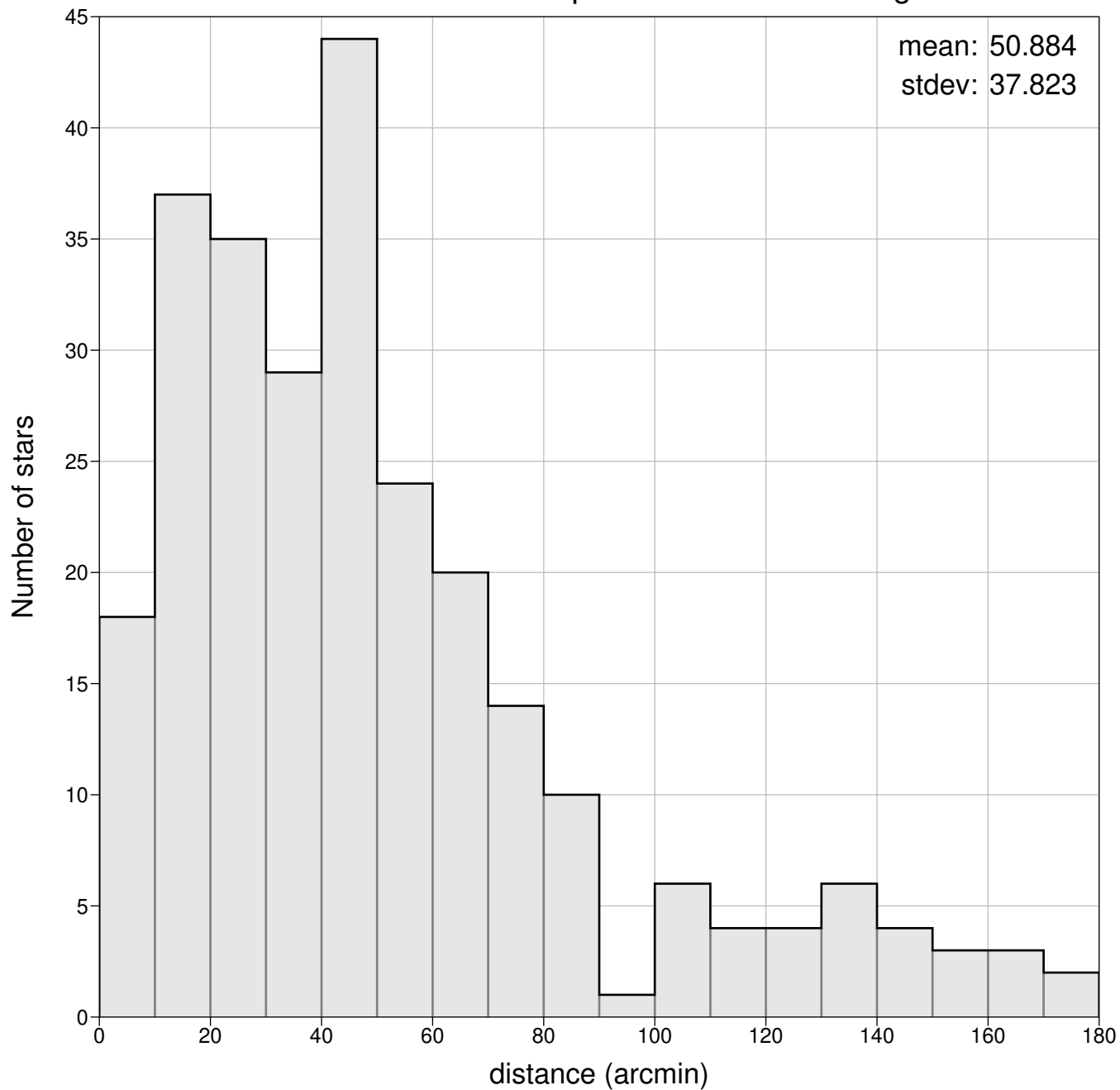
Position Error in Kepler 2a Classis Catalog
